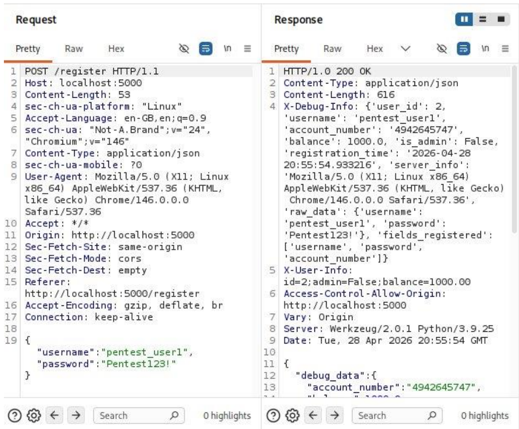
Figure 12: Decoded header value — plaintext password disclosed
