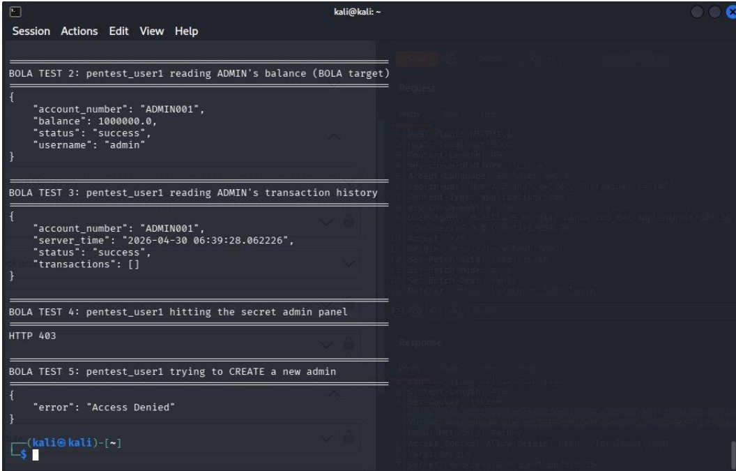
Figure 10: BOLA — attacker account accessing victim account balance successfully
