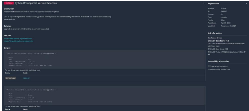
Figure 3: Nessus Plugin 148367 — Python EOL detection output (ports 80 and 5000)
