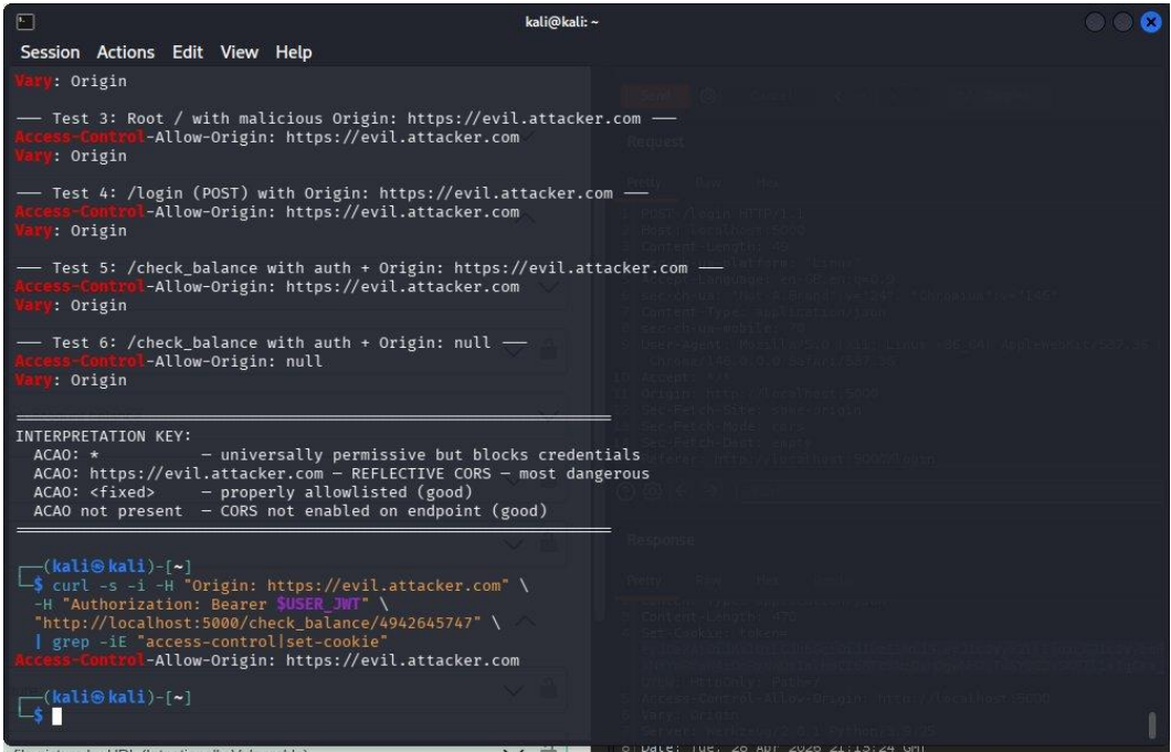
Figure 13: CORS reflection — malicious origin accepted and reflected with credentials flag
